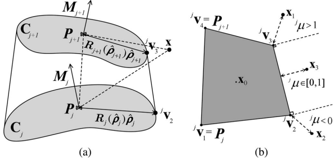
Fig. 3. (a) Basic structure of a single segment enclosed by two adjacent contours. (b) Portion of cross-sectional region extracted. Four regions to which the points \{x_0, x_1, x_2, x_3\} belong yield different distance calculations.
