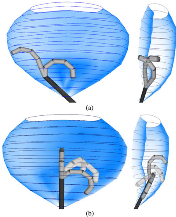
Fig. 8. (a) Four ( =\bar{n} ) control bending configurations optimized inside a complex-shaped constraint, where the robot base is inclined to one side. Two of them are bent, with even-number joint indices in front view (left), while the other two are with odd-number indices in side view (right). (b) Eight ( =\bar{n} ) optimal control bending configurations with the robot base pointing upward. The four transparent configurations are optimized in the domain of (\alpha, \beta) based on the other four configurations in solid color.
