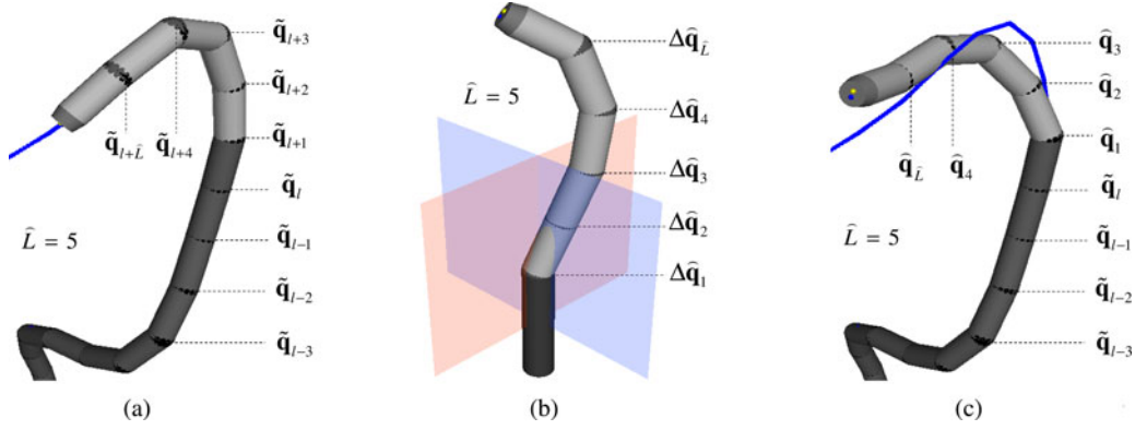
Fig. 5. (a) Configuration \tilde{\mathbf{q}} conforming to a part of the pathway along the colon below the splenic flexure. (b) Bending configuration \Delta\tilde{\mathbf{q}}(\alpha, \beta) is a combination of odd and even joint angle values; therefore, it spans a different motion plane from the ones shown in Fig. 4(c). It is also one of the optimized configurations within the spatial constraint. (c) By superposing the two configurations in (a) and (b), the resultant configuration \hat{\mathbf{q}} = \tilde{\mathbf{q}}_{l+1\dots l+\widehat{L}} + \Delta\mathbf{q}_{1\dots\widehat{L}} is obtained, which determines the bending of the last \widehat{L} links due to external manipulation. The remaining joints are fixed as \tilde{\mathbf{q}}_{1\dots l} to ensure conformance to the constraint pathway.
