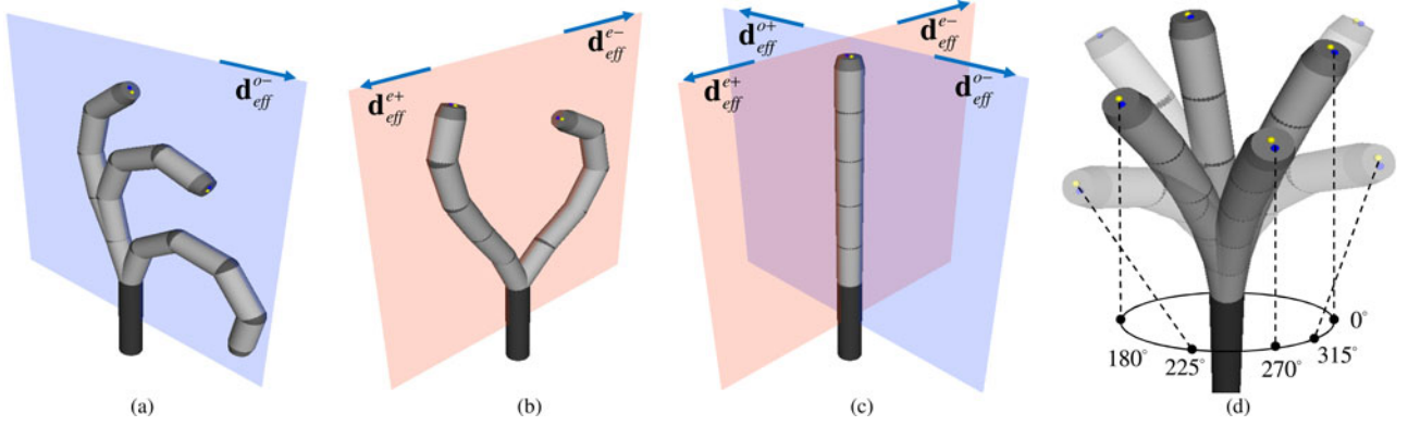
Fig. 4. (a) Three sets of variables (m, q_c) : (-0.13, -55^\circ) , (-0.23, -109.7^\circ) , and (-0.18, -119.7^\circ) generate three bending configurations with ascending curvature through the actuation of odd joint axes in one direction. (b) Two bending configurations corresponding to the actuation of even joint angles in opposite directions, parameterized as +ve: (0.31, 112.9^\circ) , -ve: (-0.11, -34.7^\circ) . (c) Motion planes spanned by even and odd joint angle actuation are perpendicular to each other. Their intersection is aligned with the robot axis in the straight configuration \widehat{\mathbf{q}} = \vec{0} . Four primitive bending directions are indicated. (d) Four primitive bending configurations with (m, q_c) = (0, \pm 5^\circ) are represented in solid color. The other four configurations displayed in semitransparent color are generated between the four primitive configurations by assigning (\alpha, \beta) = (0.25, 3.35) .
