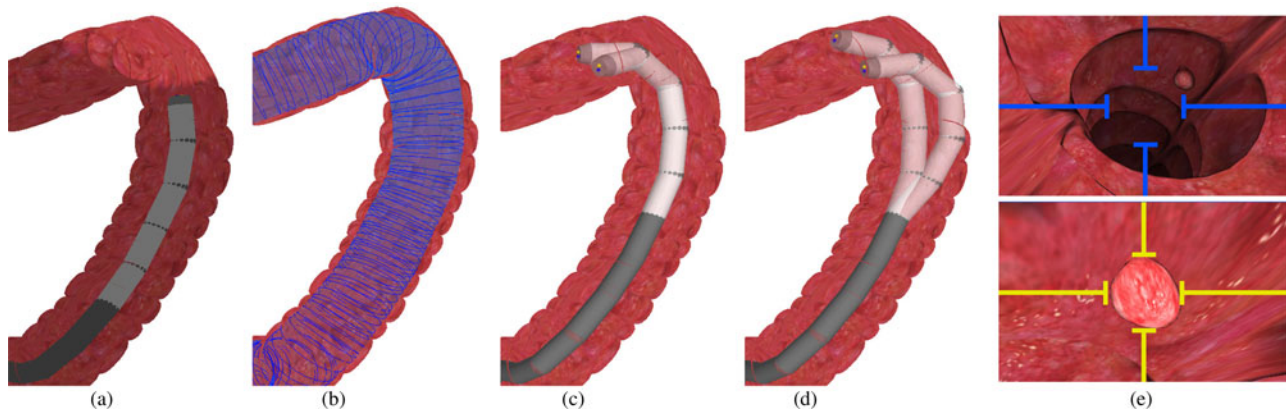
Fig. 9. (a) Robot conforms along the centerline of the CT colon model used to simulate colonoscopy. Endoscopic lighting is also simulated and projected on the splenic flexure. (b) Fifty ( =N_C ) circular contours with varied radii are fitted manually to the whole colon model. One hundred and ninety-seven ( =\tilde{N}_C ) contours are interpolated to smoothen the constraint pathway (in blue). (c) and (d) Four control bending configurations optimized inside the flexure for viewing polyps on the transverse colon wall. (e) Polyp is clearly visualized within the camera view under sufficient endoscopic lighting. The color of the aiming marker is changed gradually based on the targeting accuracy. (Top, in blue): Out of the viewing range. (Bottom in sharp yellow): Very accurate targeting.
