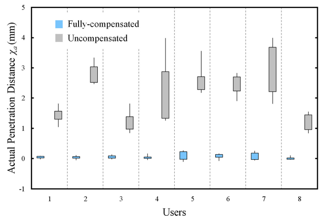
Fig. 9. A box plot showing thresholds for the actual distance penetrated by the tool tip following the user's indication that they had perceived the active constraint for both fully compensated and uncompensated cases.
