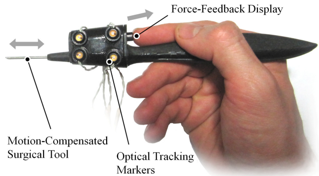
Fig. 1. A photograph of the hand-held device illustrating its key features of motion compensation and force-feedback.
