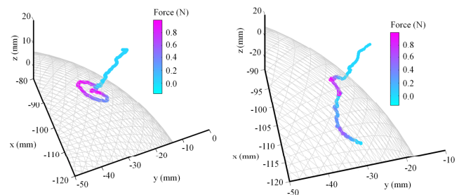
Fig. 7. Plot showing the actual tool tip position P_a in a free hand palpation of a spherical active constraint for both rigid (left) and soft (right) active constraints in which the tool tip motion is fully compensated and scaled respectively.
