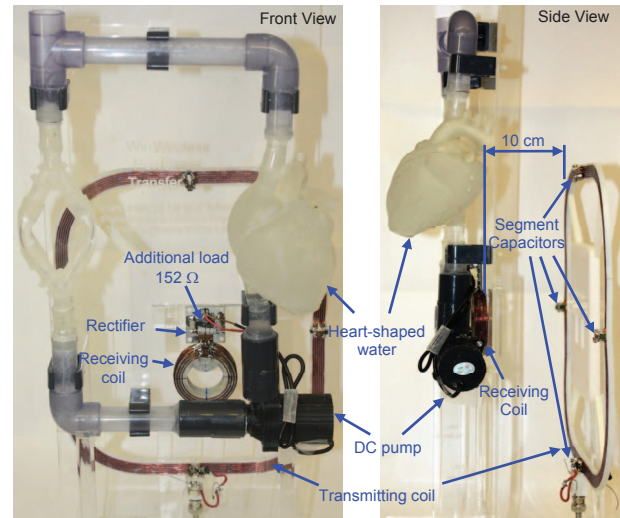
Fig. 10. Front and side views of the wirelessly powered circulatory model.
