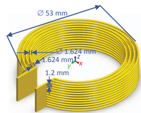
Fig. 6. The energy receiving coil.
